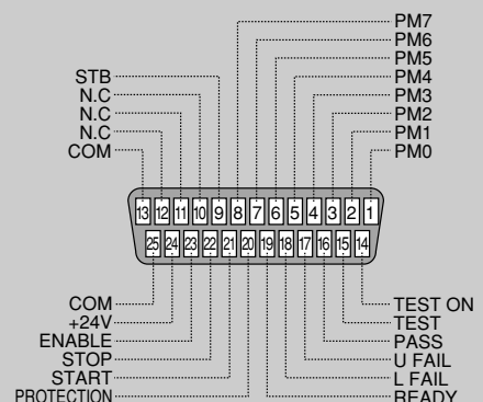
[Pin Configuration for the SIGNAL I/O Connector]
