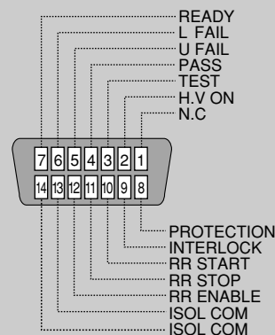
[Pin Configuration for the SIGNAL I/O Connector]
